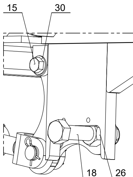
DETAIL A SCALE 1 : 4
