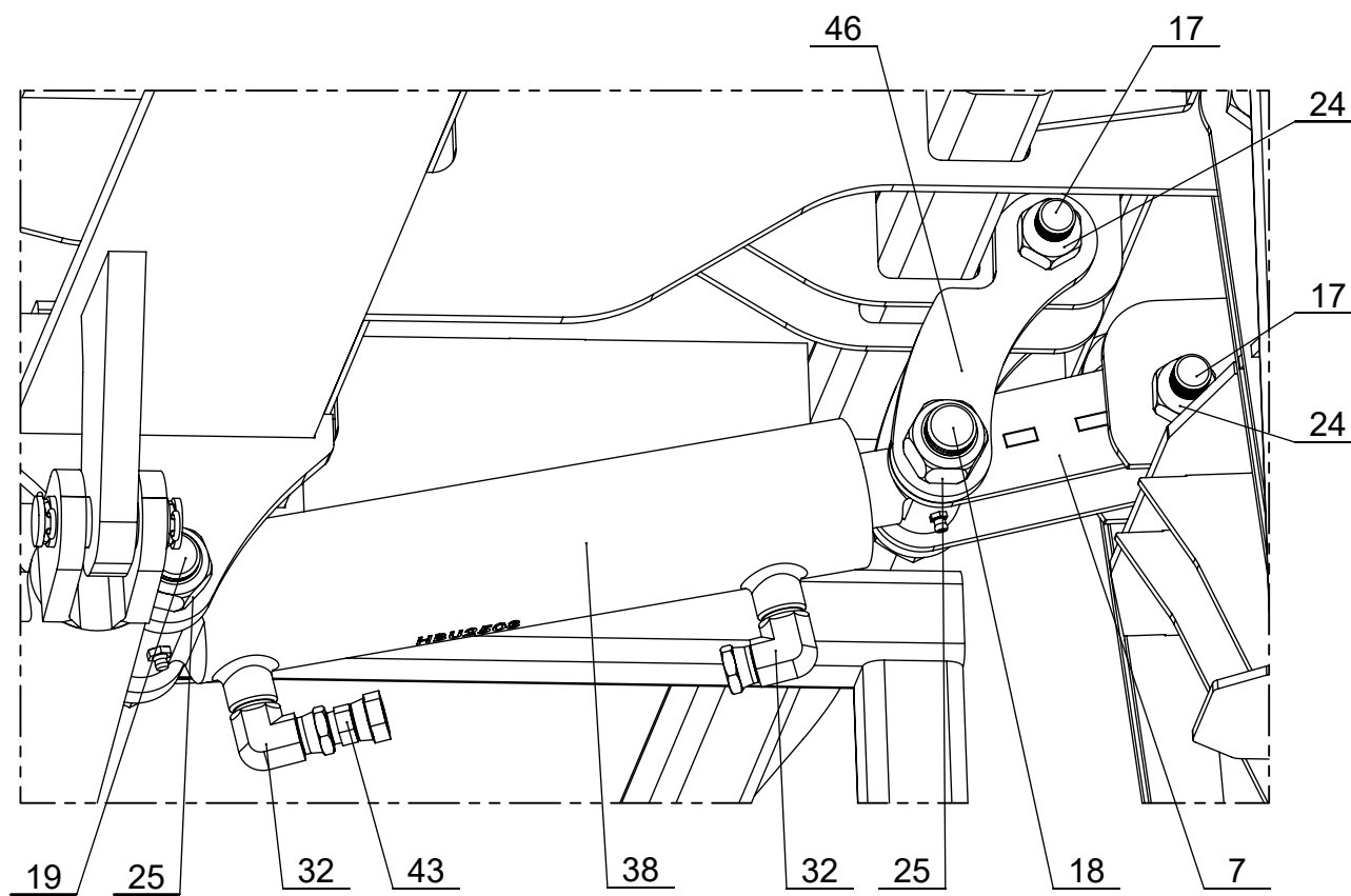
DETAIL B SCALE 1 : 4
