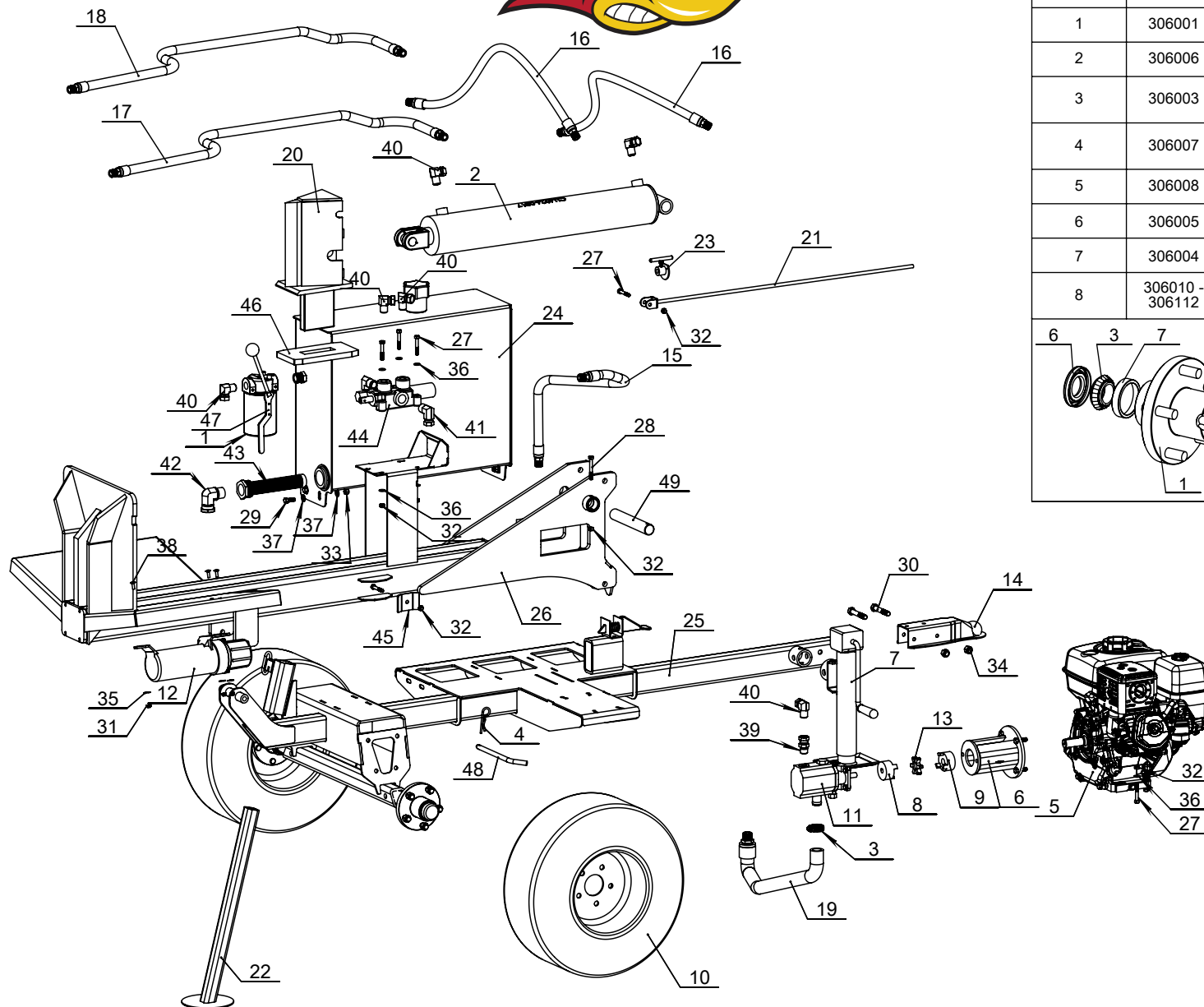
Hub & Axles 1250 lbs 5 nuts
