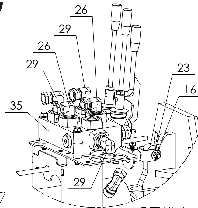
DETAIL A SCALE 1 : 5
