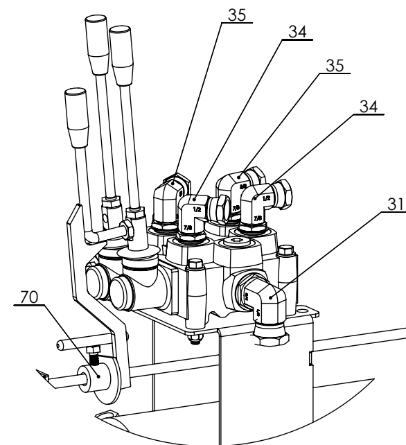
DETAIL B SCALE 1 : 5
