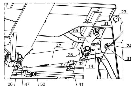
DETAIL C SCALE 1 : 6
