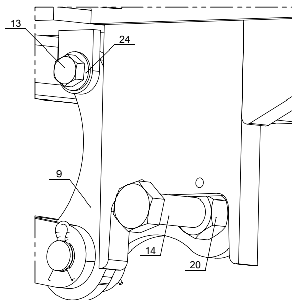
DETAIL C SCALE 1 : 3
