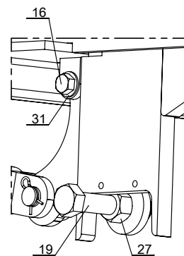
DETAIL D SCALE 1 : 6
